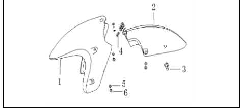
F-1 Front Fender Assy
