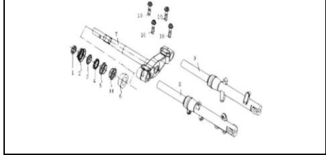
F-2 Front Fork
